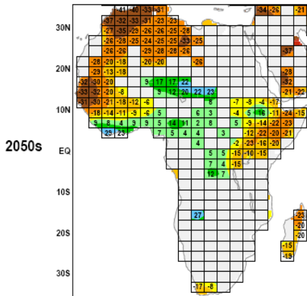
Projected Precipitation - June-July-August >3°C by mid-century
